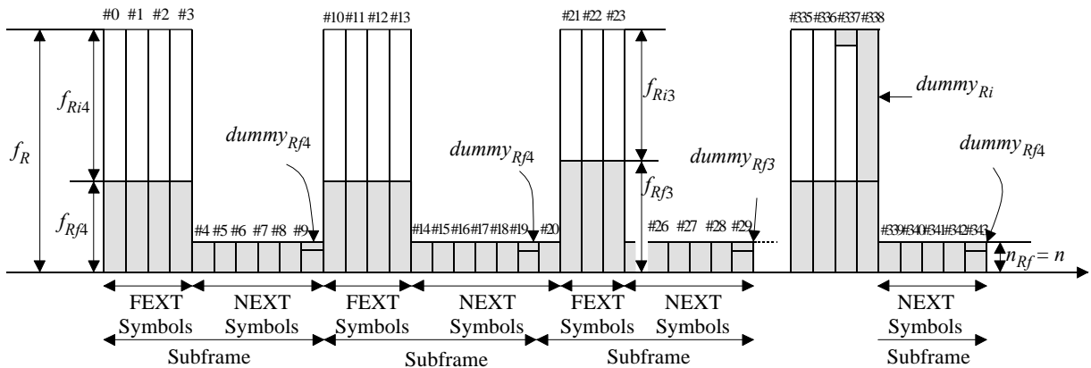
Figure Q.12/G.992.1 – Bit distribution for Rate Converter under Dual latency and Dual Bitmap mode
