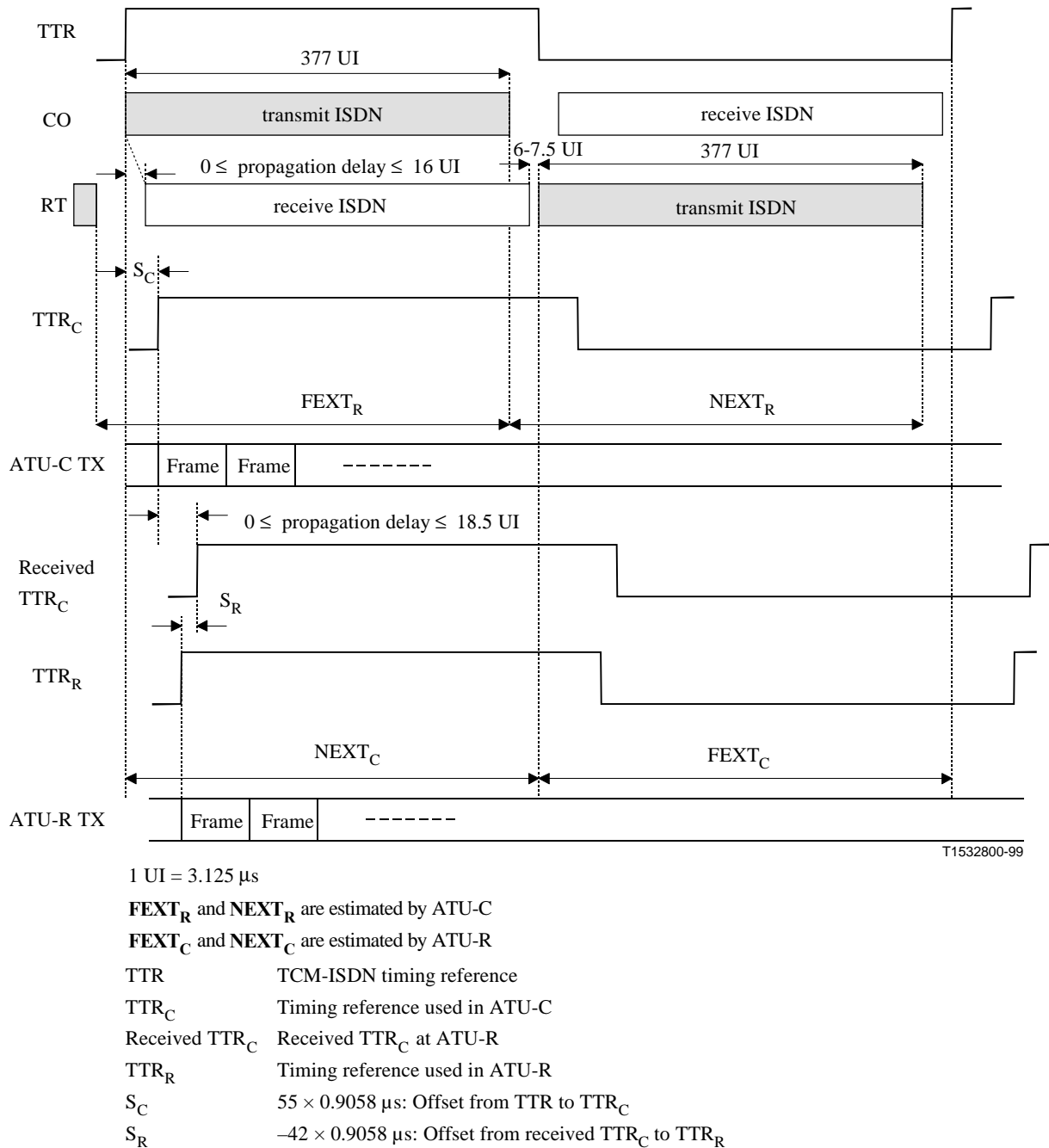
Figure Q.5/G.992.1 – Timing chart of the TCM-ISDN crosstalk
